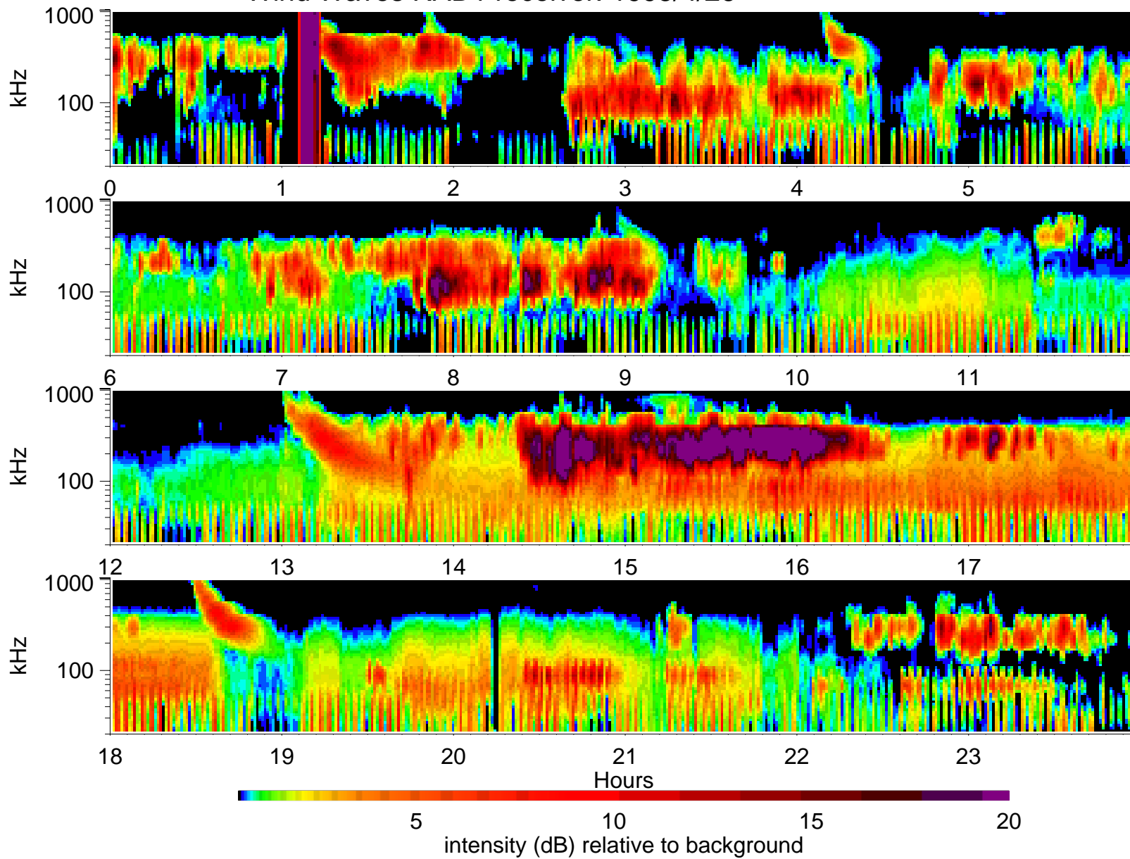
Wind Waves RAD1 receiver: 1995/4/26
