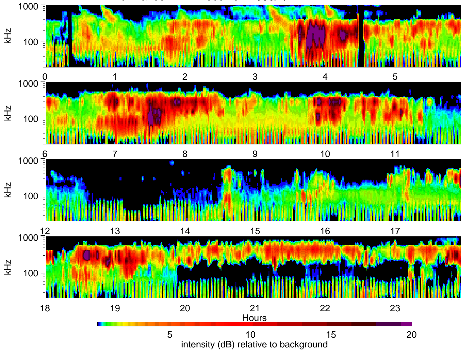
Wind Waves RAD1 receiver: 1995/4/24
