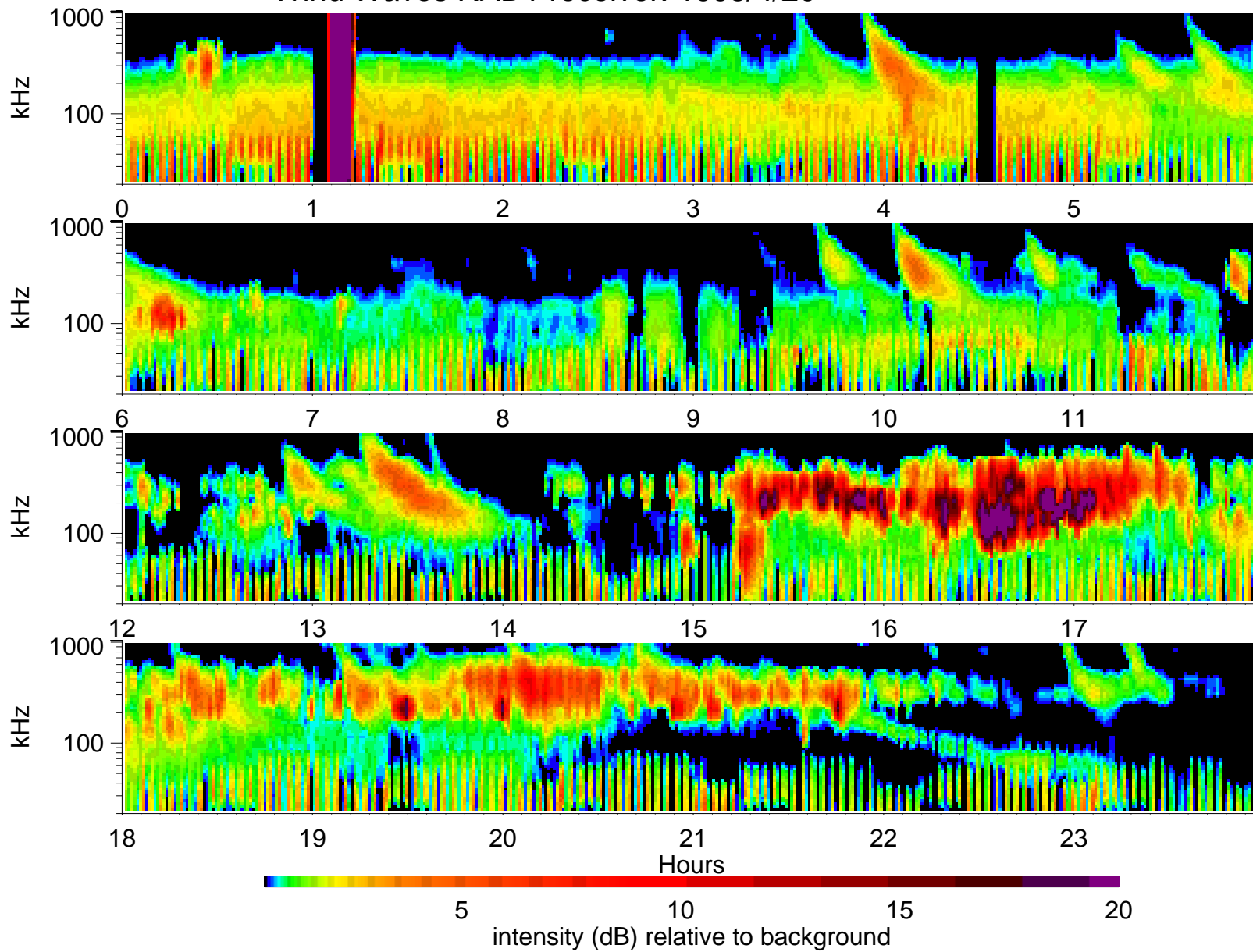
Wind Waves RAD1 receiver: 1995/4/20
