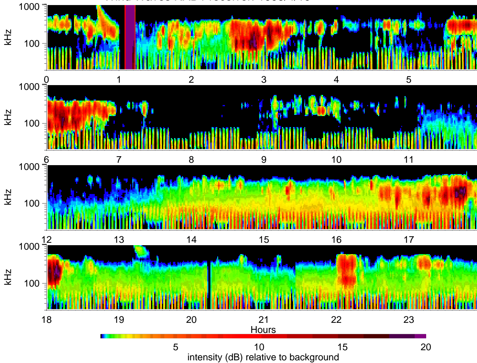
Wind Waves RAD1 receiver: 1995/4/19
