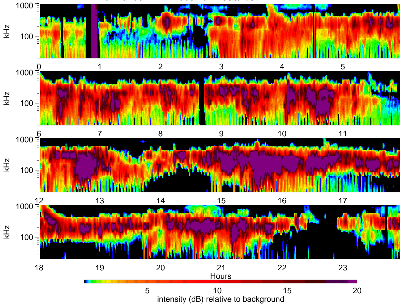
Wind Waves RAD1 receiver: 1995/4/8
