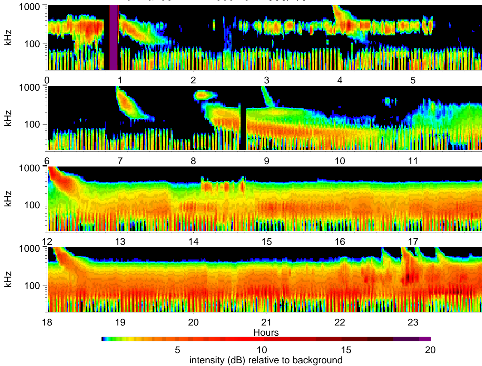
Wind Waves RAD1 receiver: 1995/4/6
