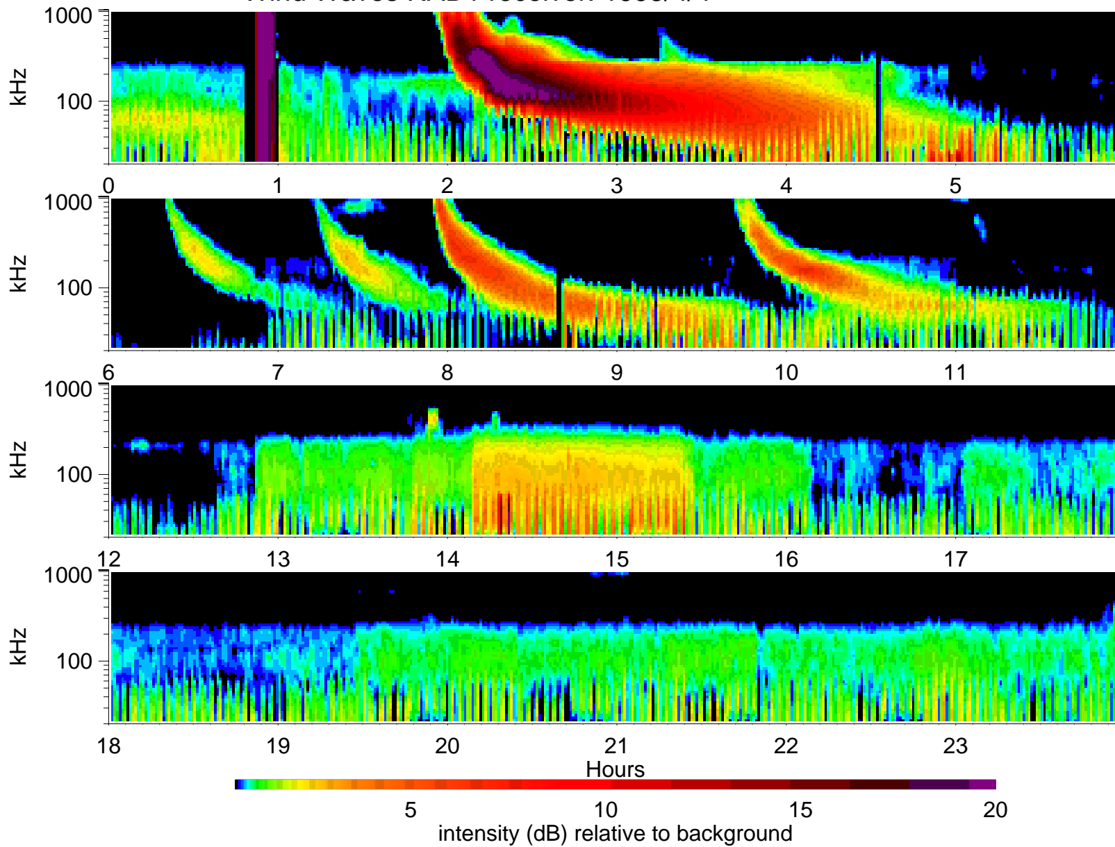
Wind Waves RAD1 receiver: 1995/4/4
