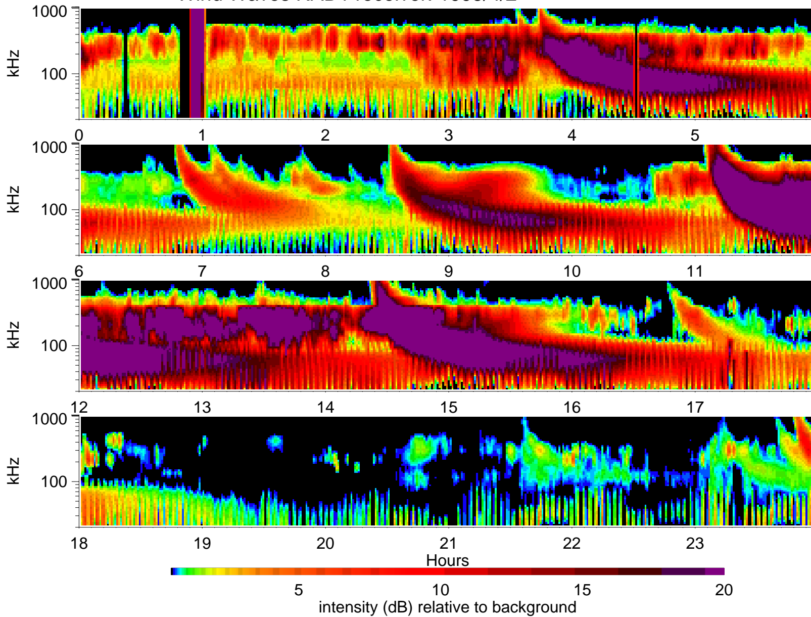
Wind Waves RAD1 receiver: 1995/4/2
