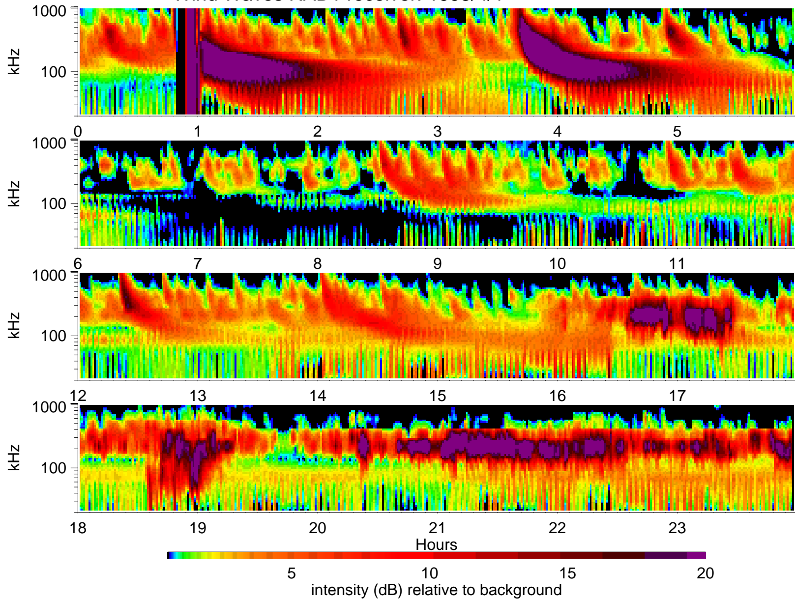
Wind Waves RAD1 receiver: 1995/4/1
