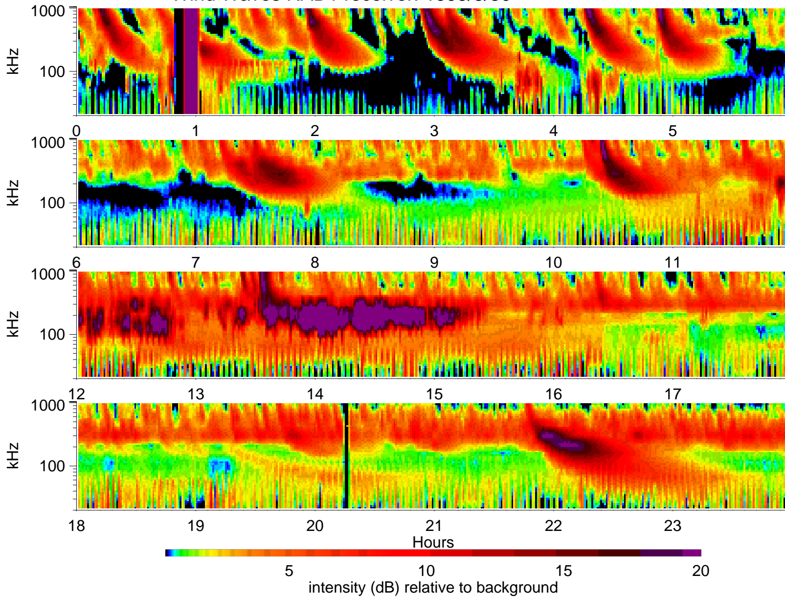
Wind Waves RAD1 receiver: 1995/3/30
