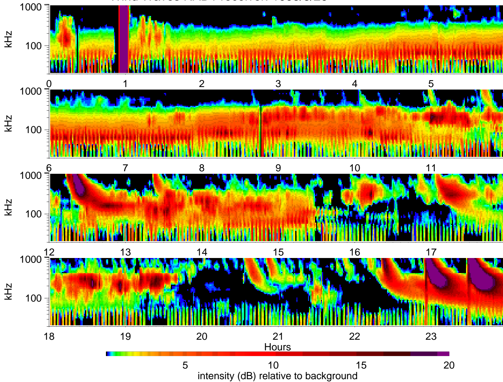
Wind Waves RAD1 receiver: 1995/3/26
