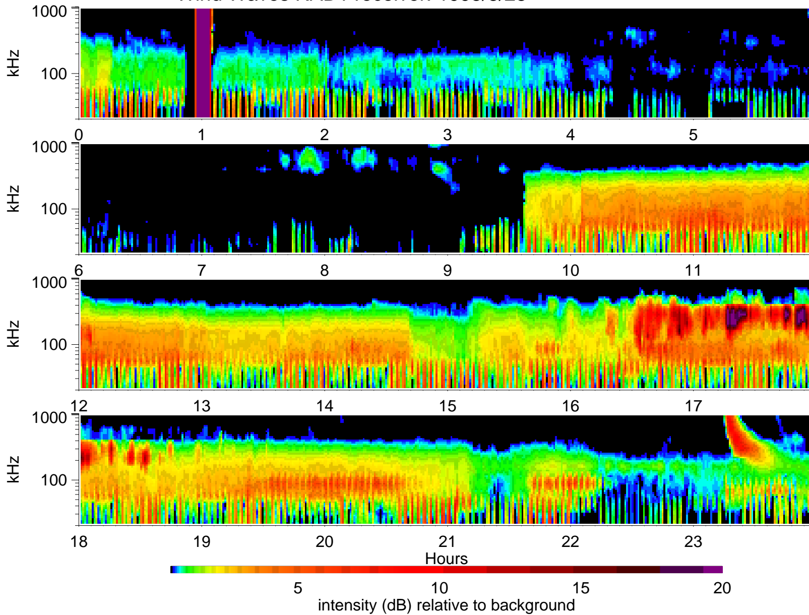
Wind Waves RAD1 receiver: 1995/3/23
