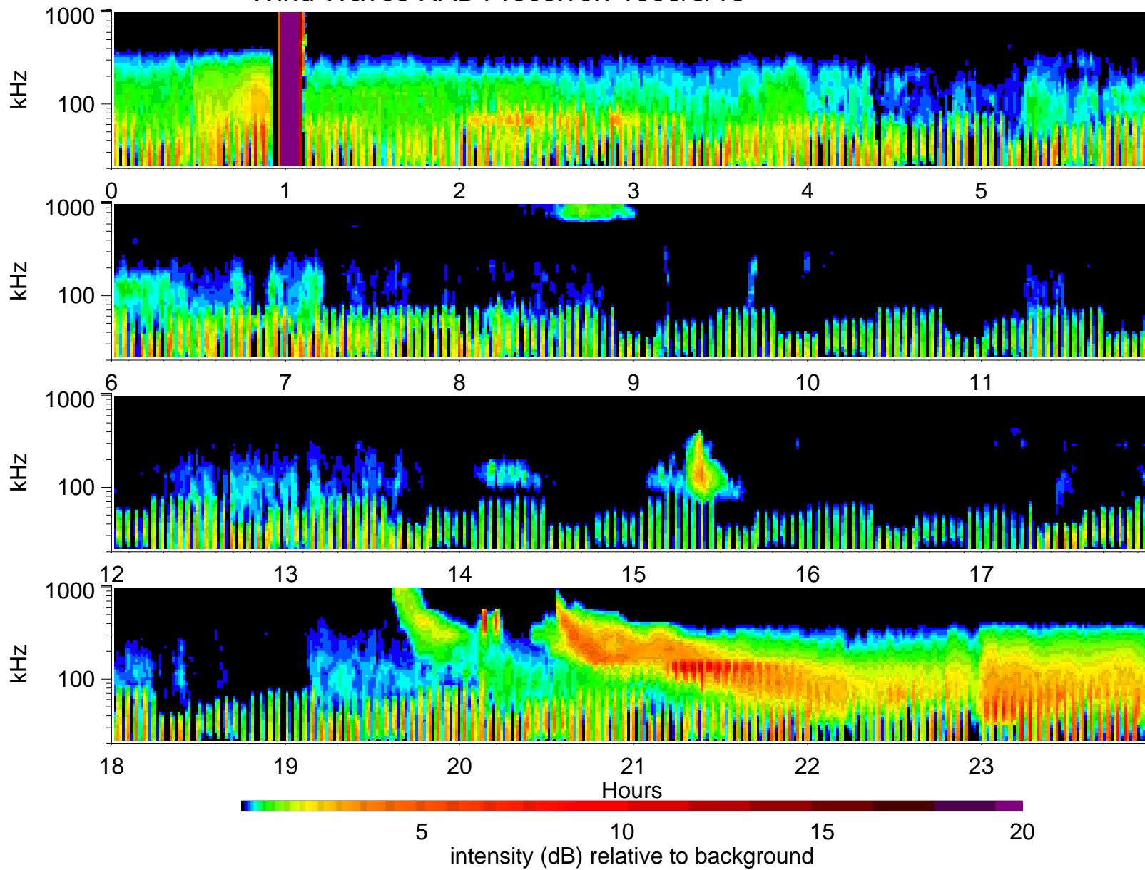
Wind Waves RAD1 receiver: 1995/3/18
