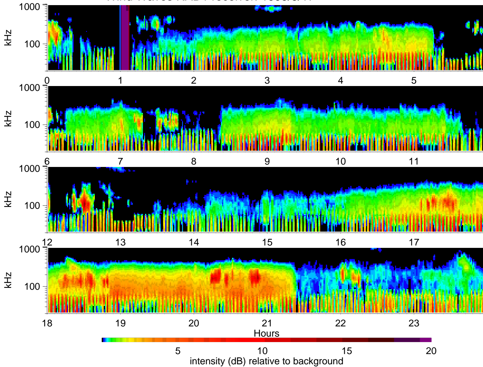
Wind Waves RAD1 receiver: 1995/3/17
