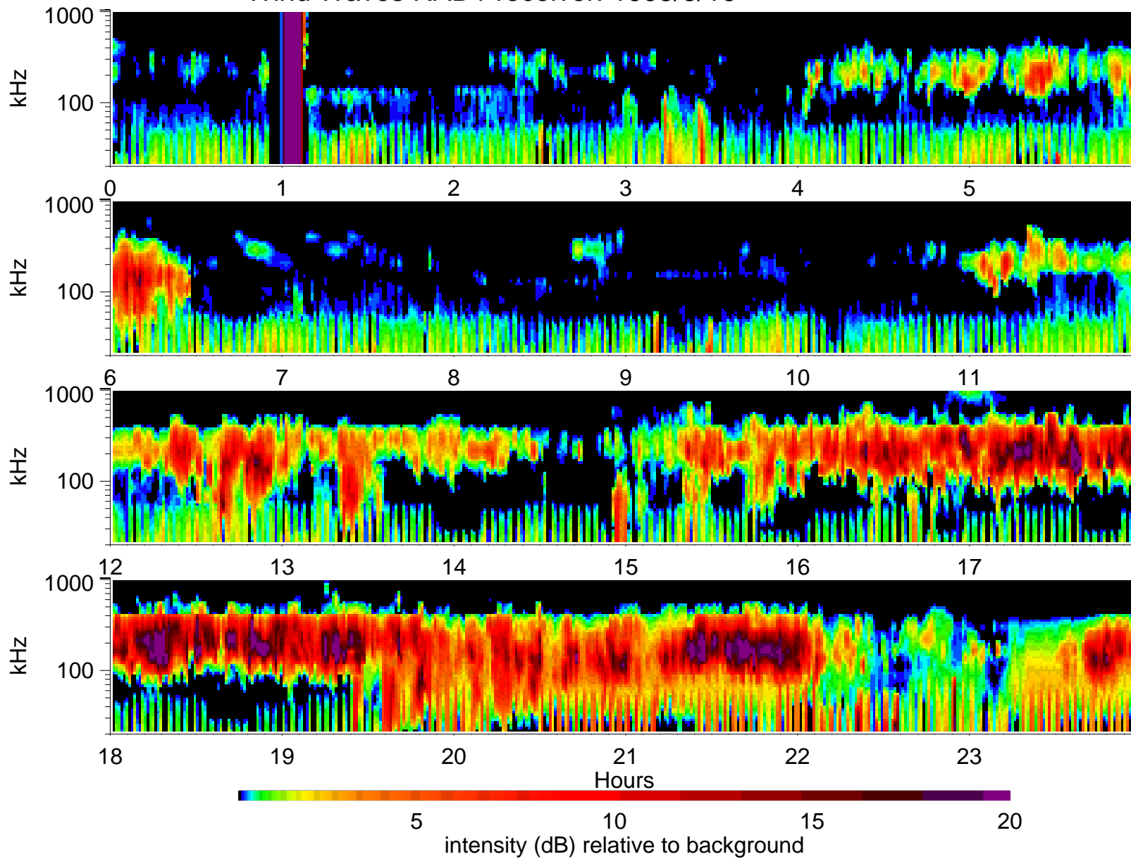
Wind Waves RAD1 receiver: 1995/3/16
