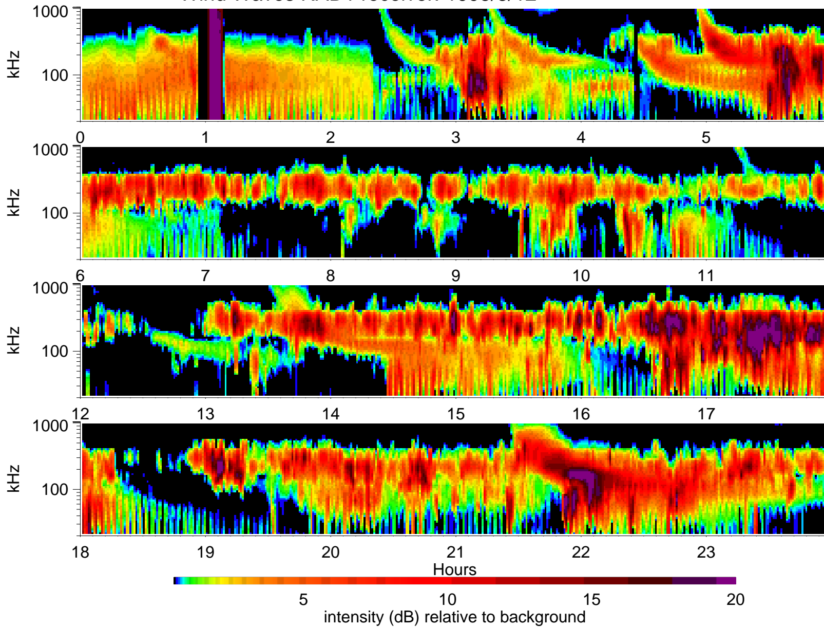
Wind Waves RAD1 receiver: 1995/3/12
