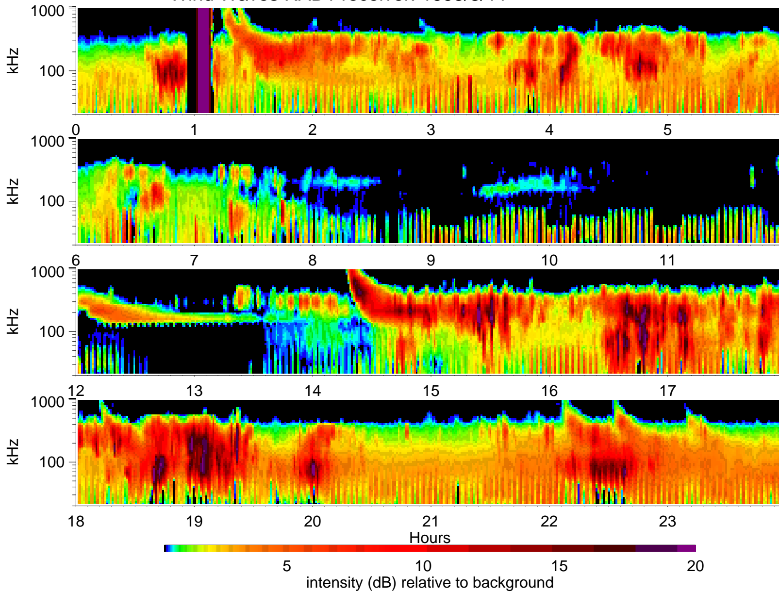
Wind Waves RAD1 receiver: 1995/3/11
