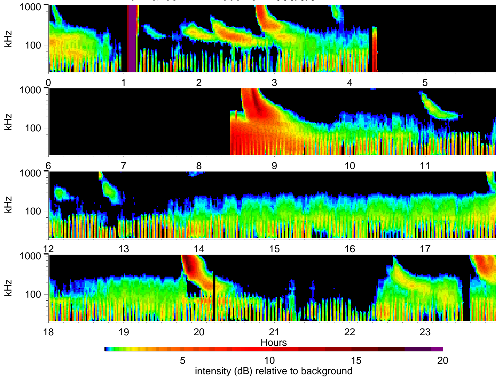
Wind Waves RAD1 receiver: 1995/3/8
