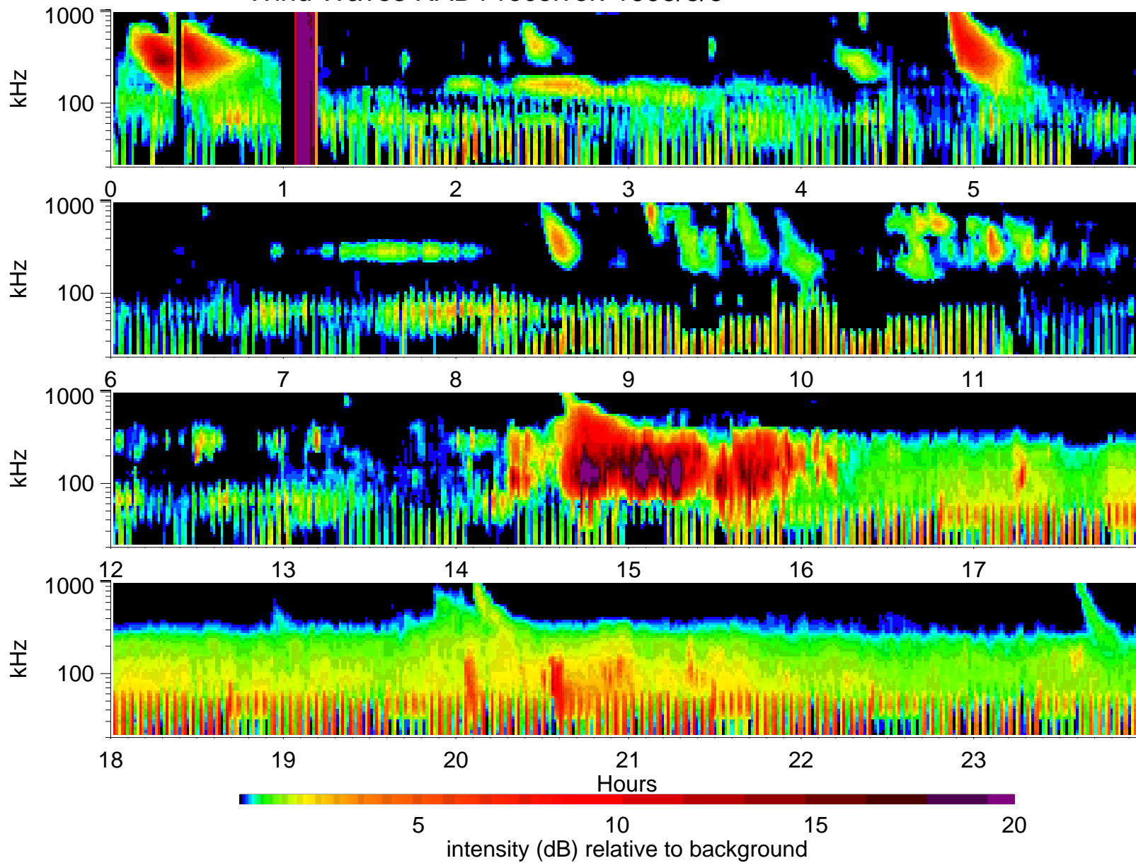
Wind Waves RAD1 receiver: 1995/3/5
