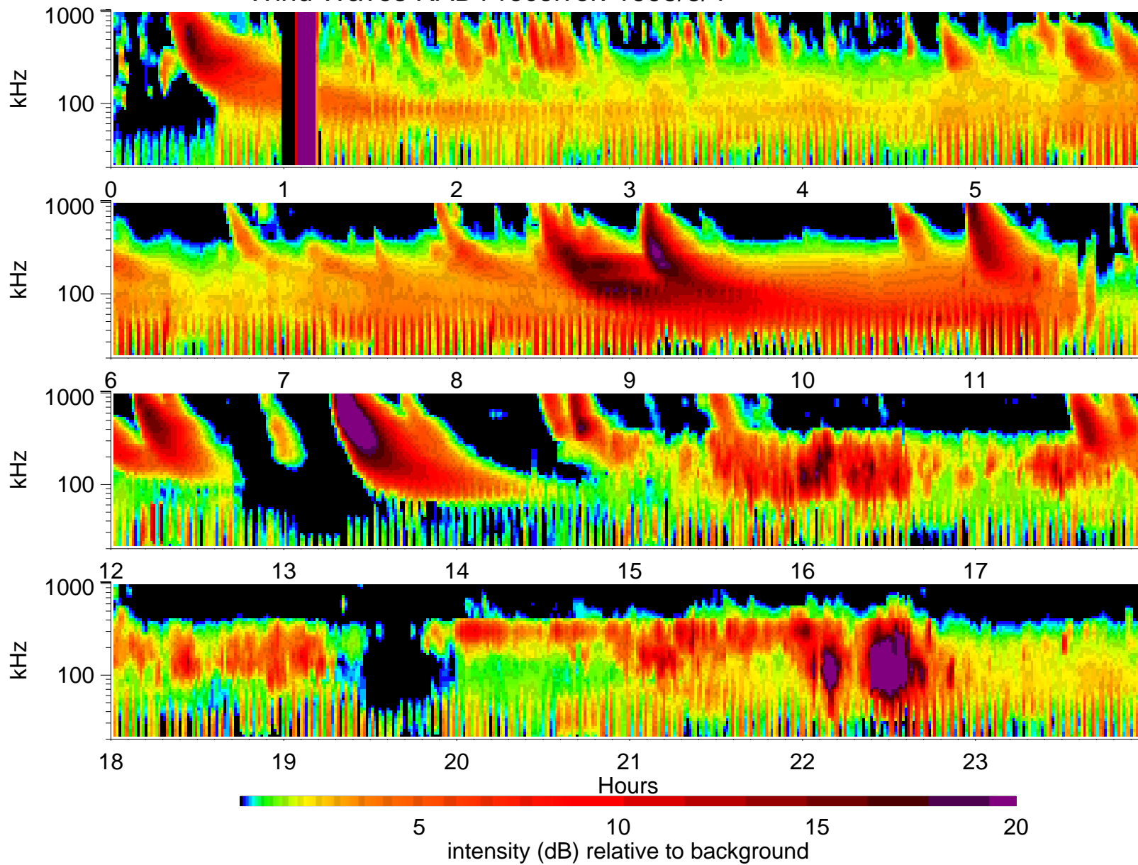
Wind Waves RAD1 receiver: 1995/3/4
