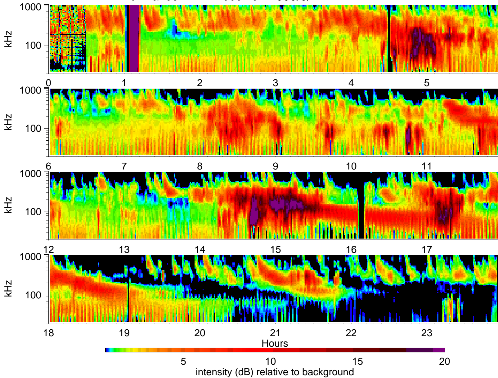
Wind Waves RAD1 receiver: 1995/3/2
