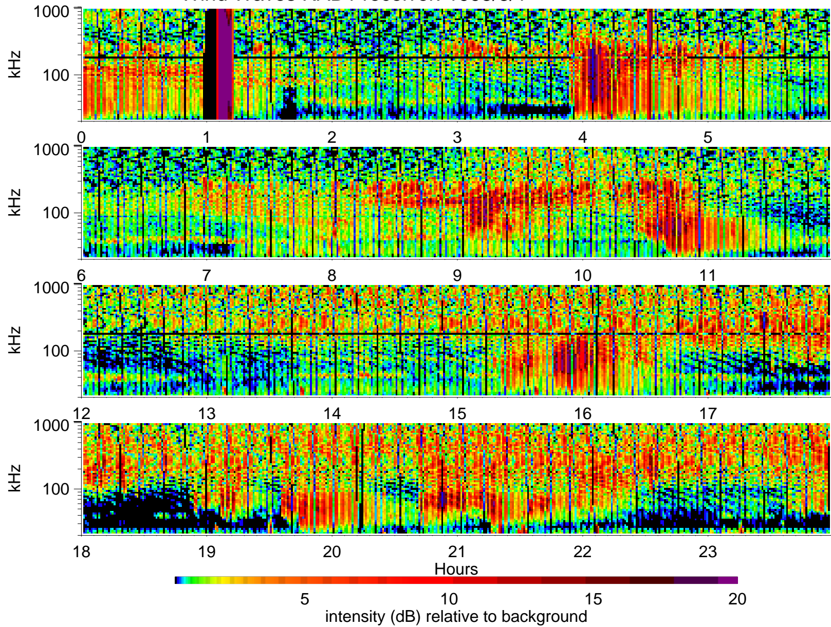
Wind Waves RAD1 receiver: 1995/3/1
