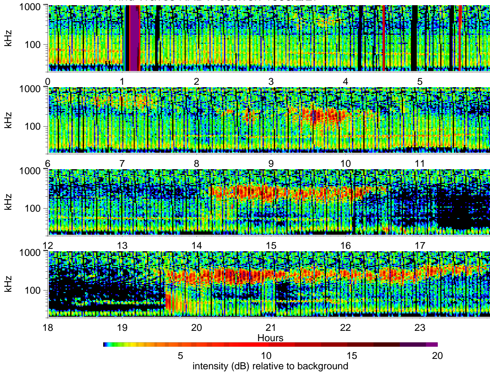
Wind Waves RAD1 receiver: 1995/2/27
