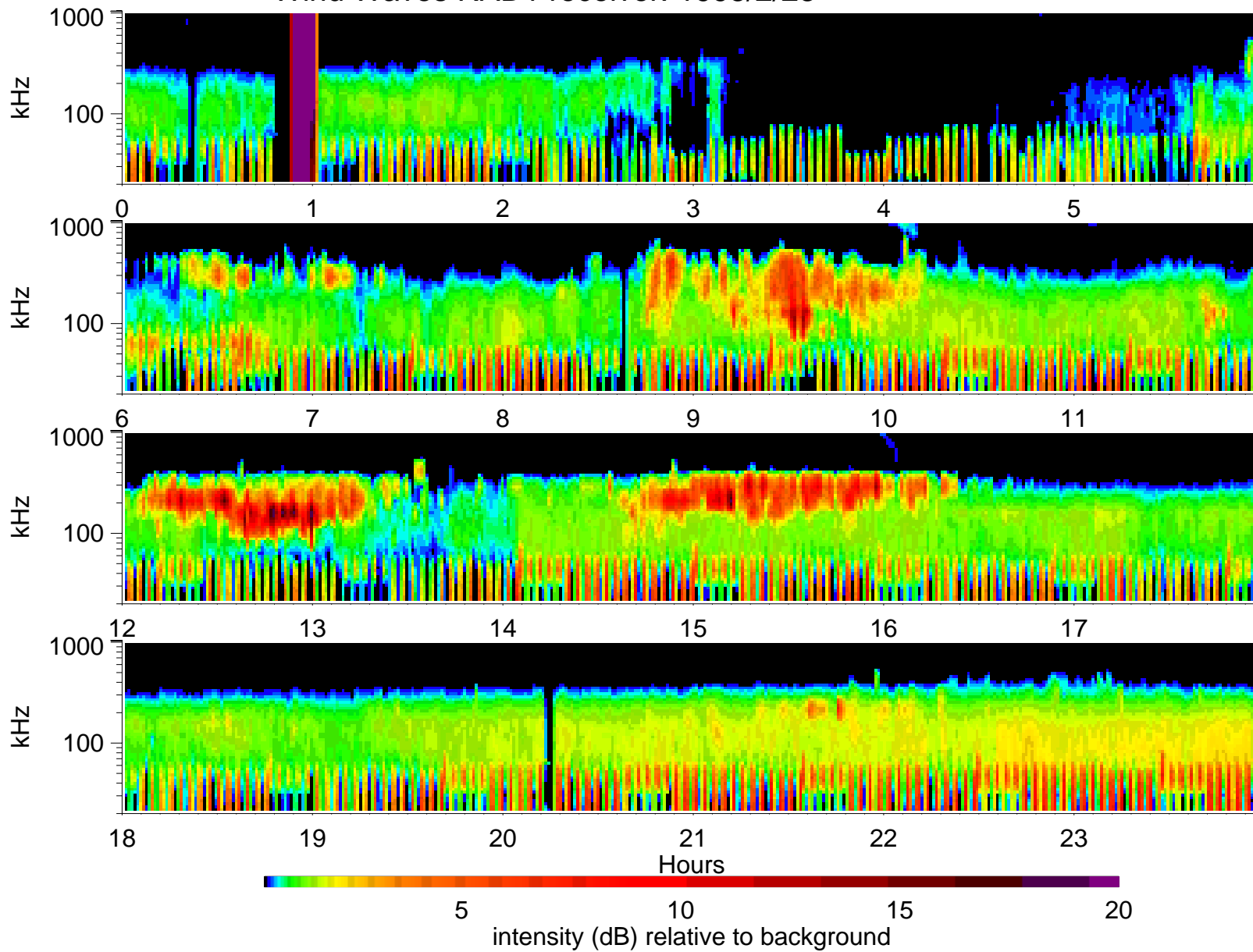
Wind Waves RAD1 receiver: 1995/2/23
