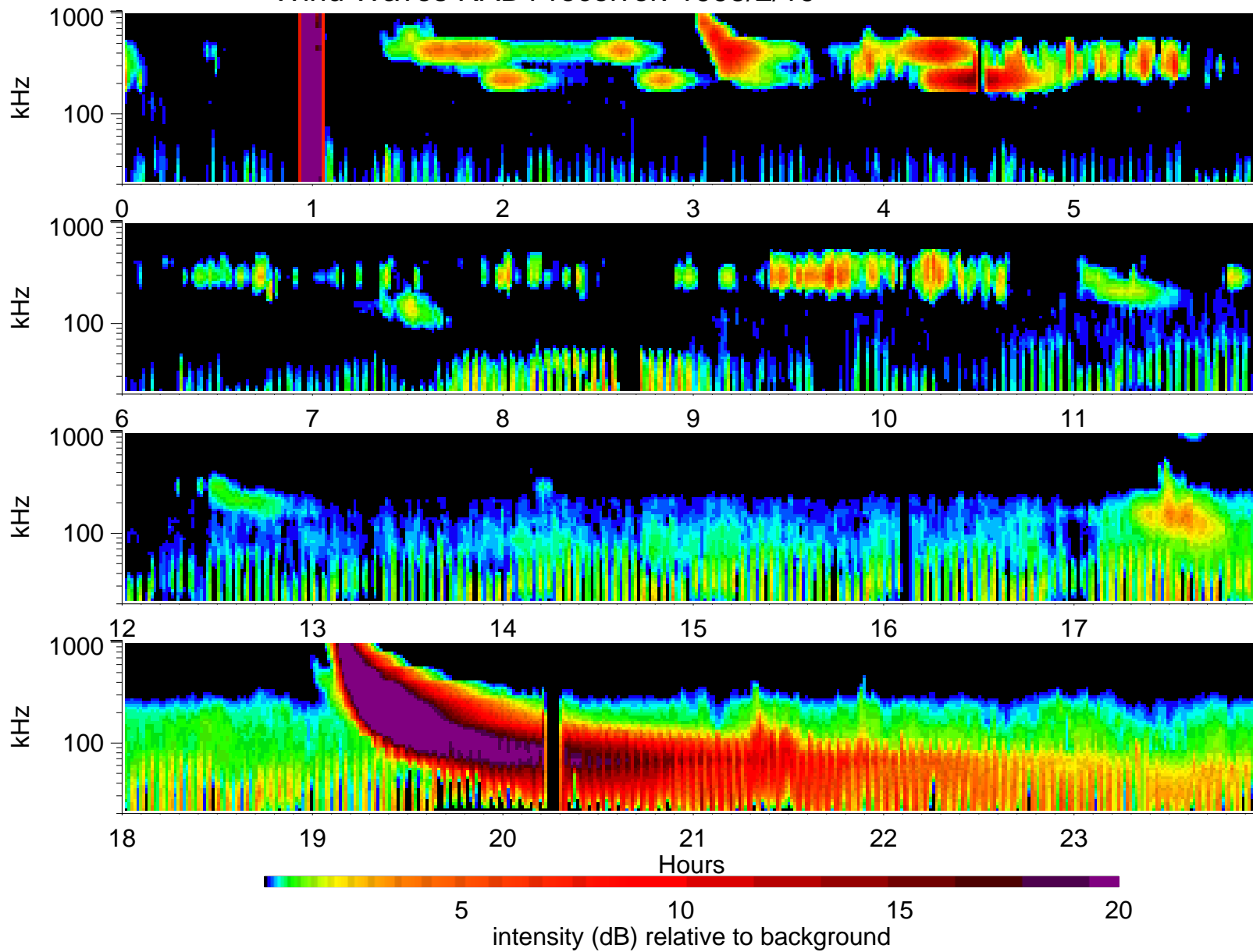
Wind Waves RAD1 receiver: 1995/2/19
