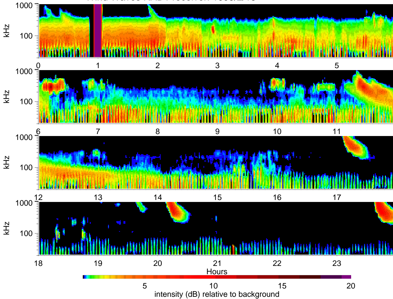
Wind Waves RAD1 receiver: 1995/2/18
