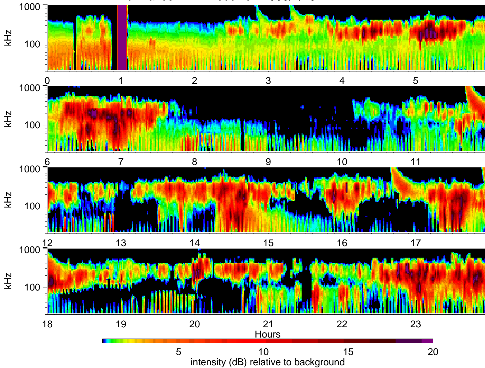
Wind Waves RAD1 receiver: 1995/2/13
