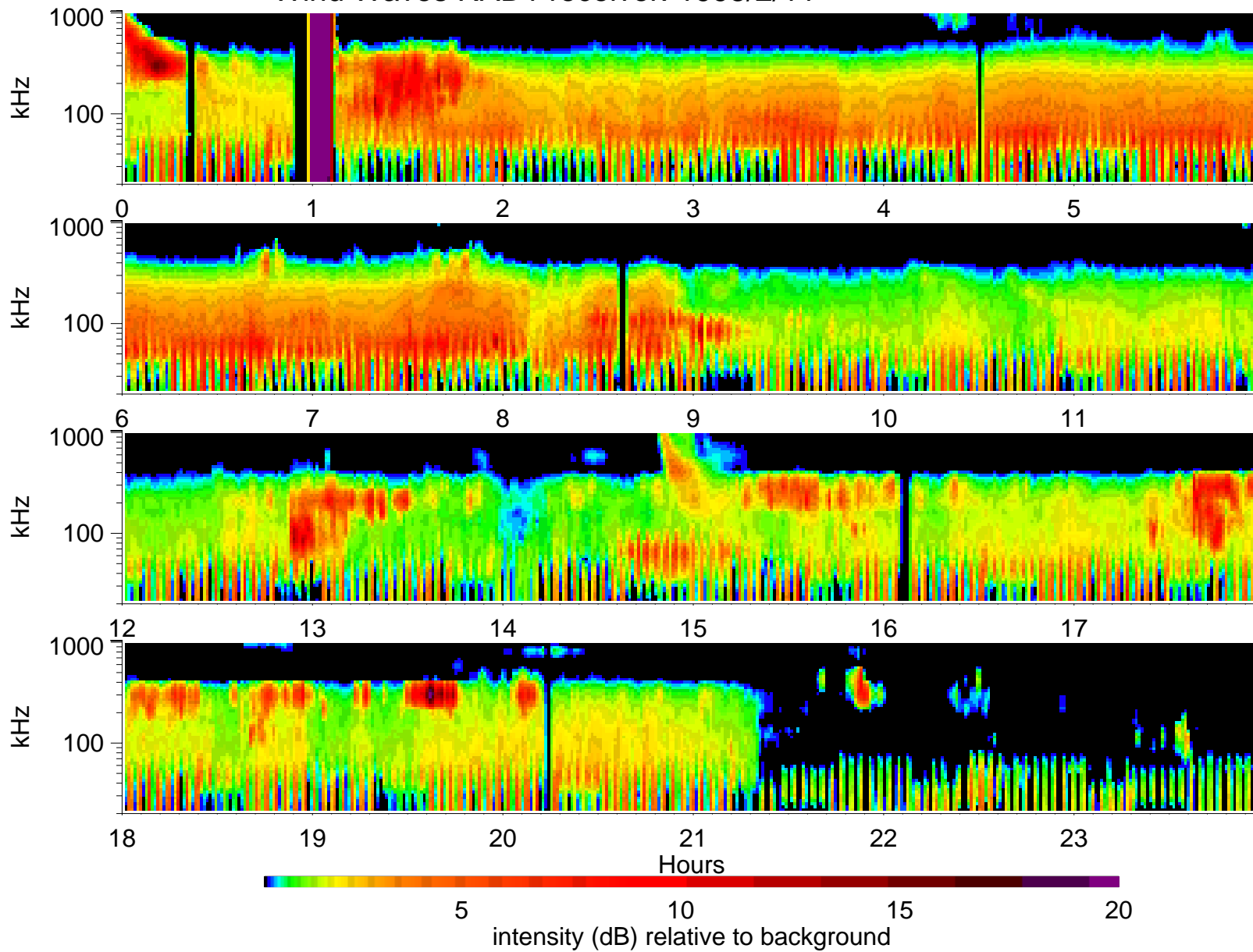
Wind Waves RAD1 receiver: 1995/2/11
