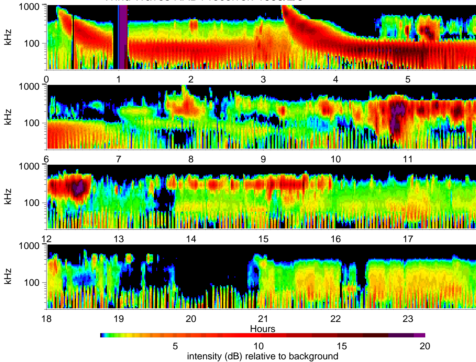
Wind Waves RAD1 receiver: 1995/2/8
