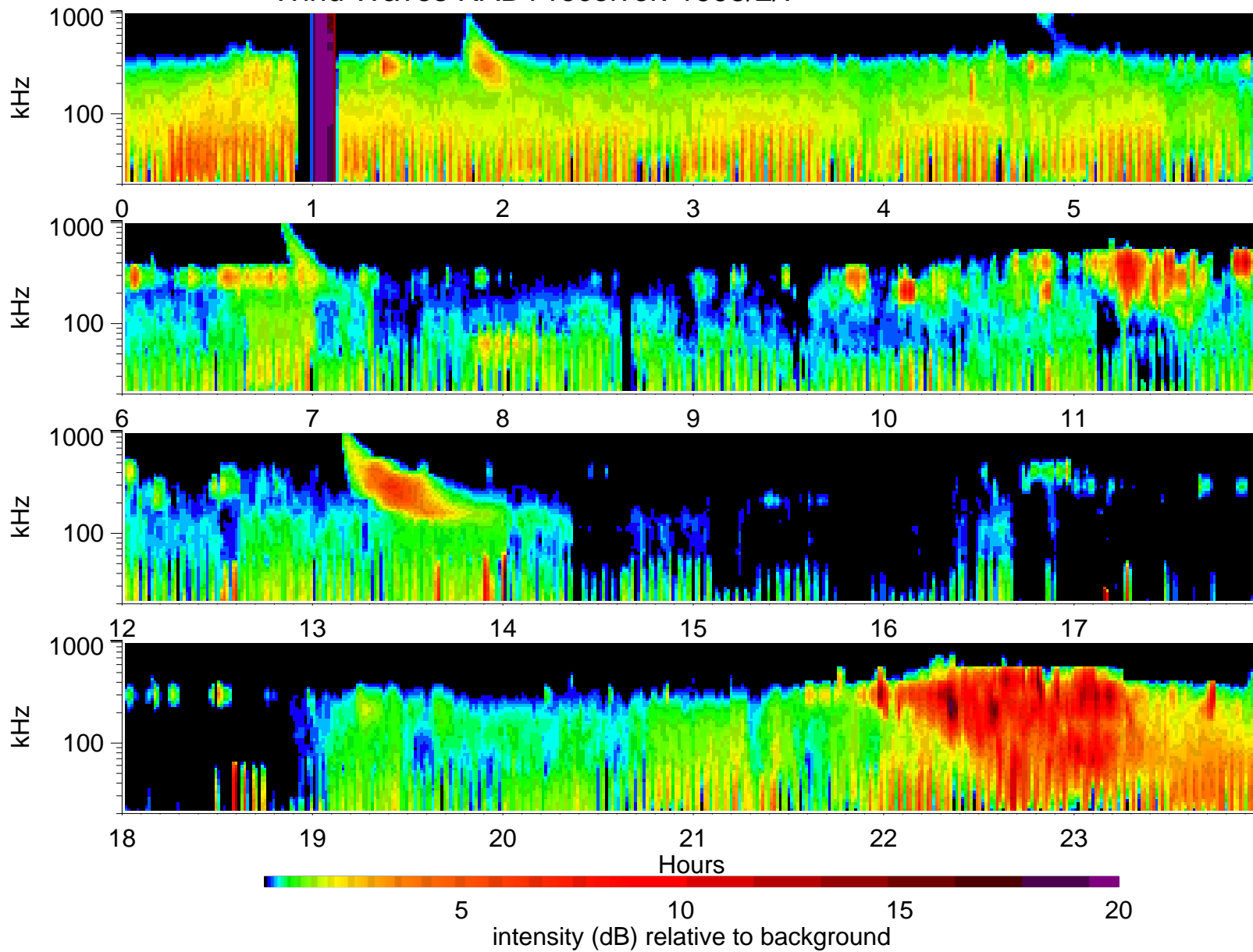
Wind Waves RAD1 receiver: 1995/2/7
