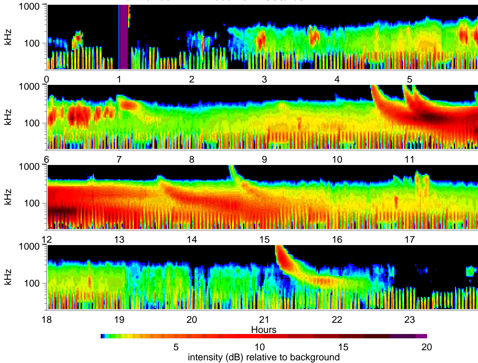
Wind Waves RAD1 receiver: 1995/2/6
