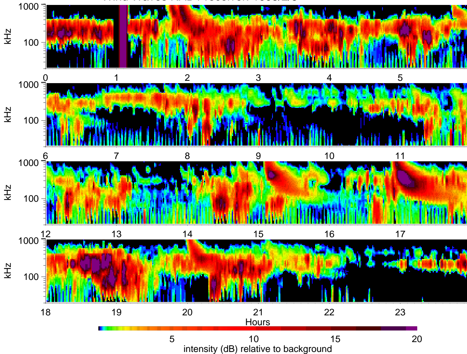
Wind Waves RAD1 receiver: 1995/2/3
