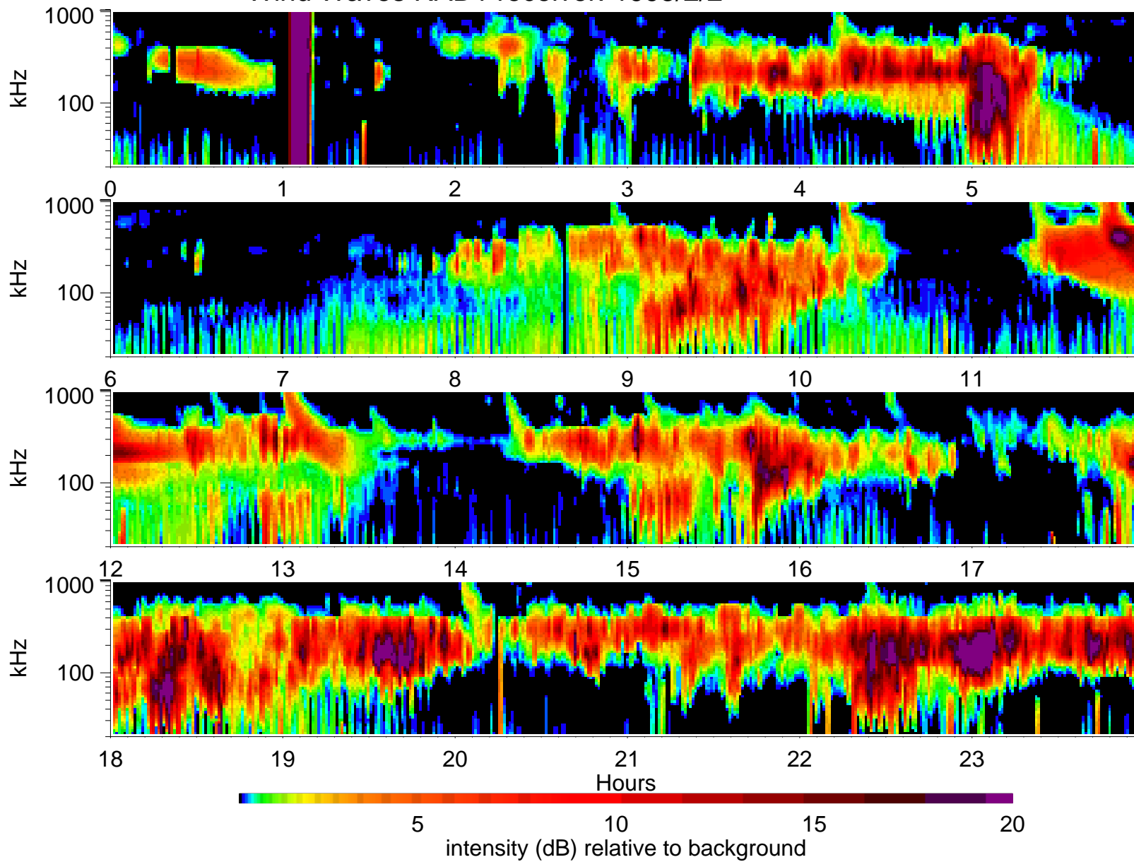
Wind Waves RAD1 receiver: 1995/2/2
