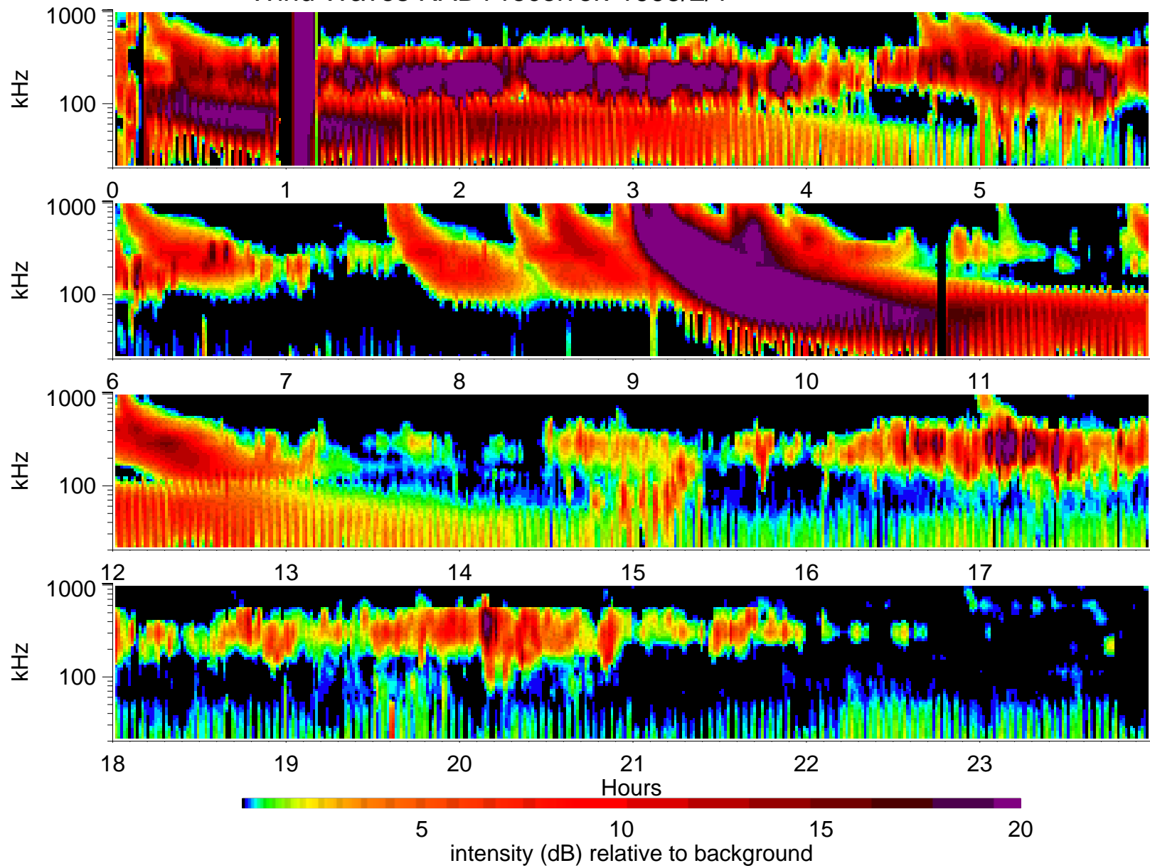
Wind Waves RAD1 receiver: 1995/2/1
