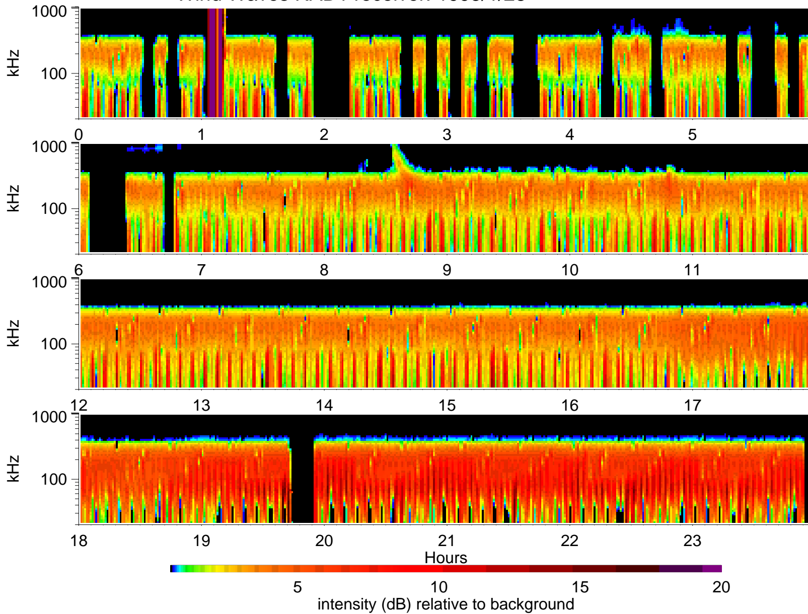
Wind Waves RAD1 receiver: 1995/1/28
