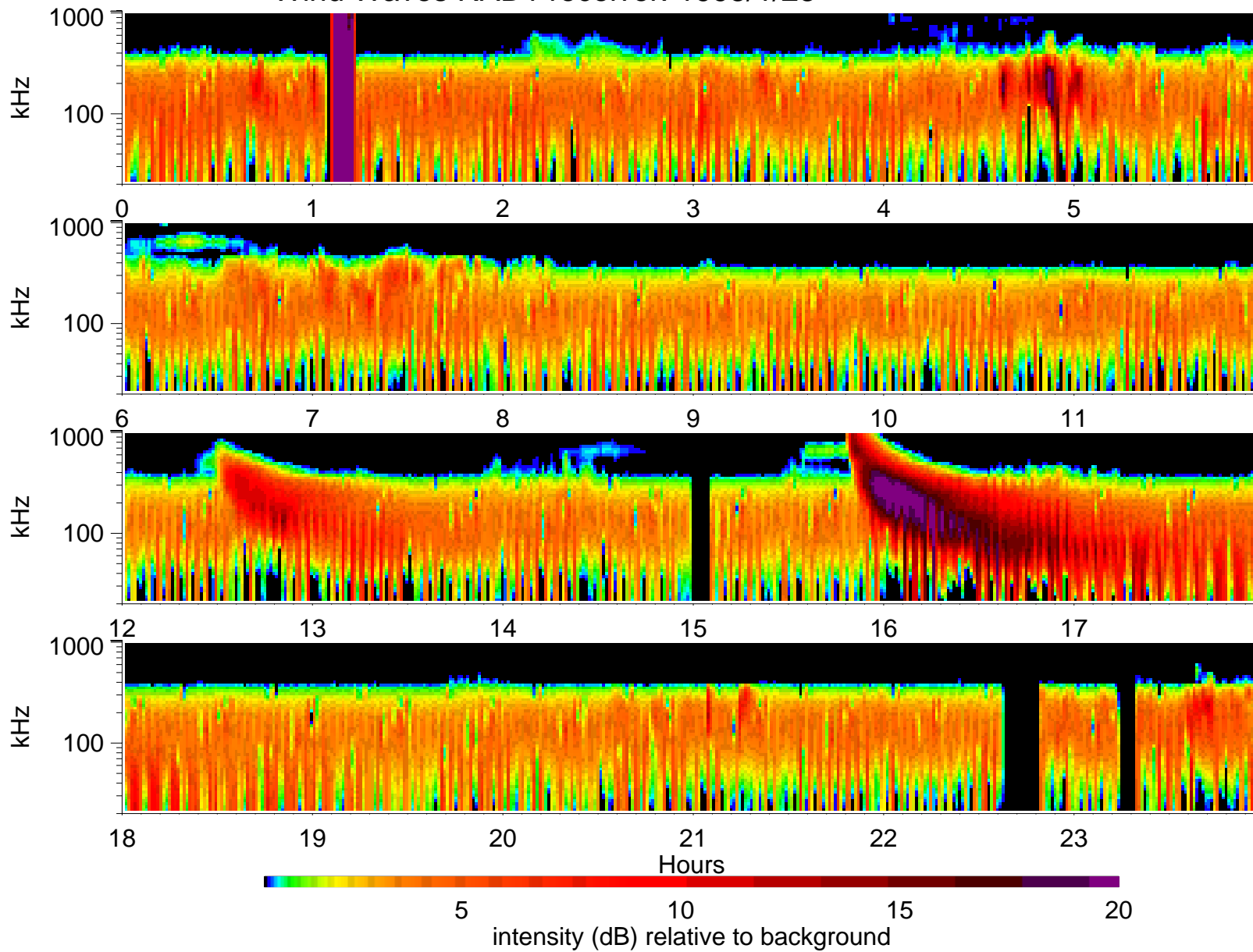
Wind Waves RAD1 receiver: 1995/1/23
