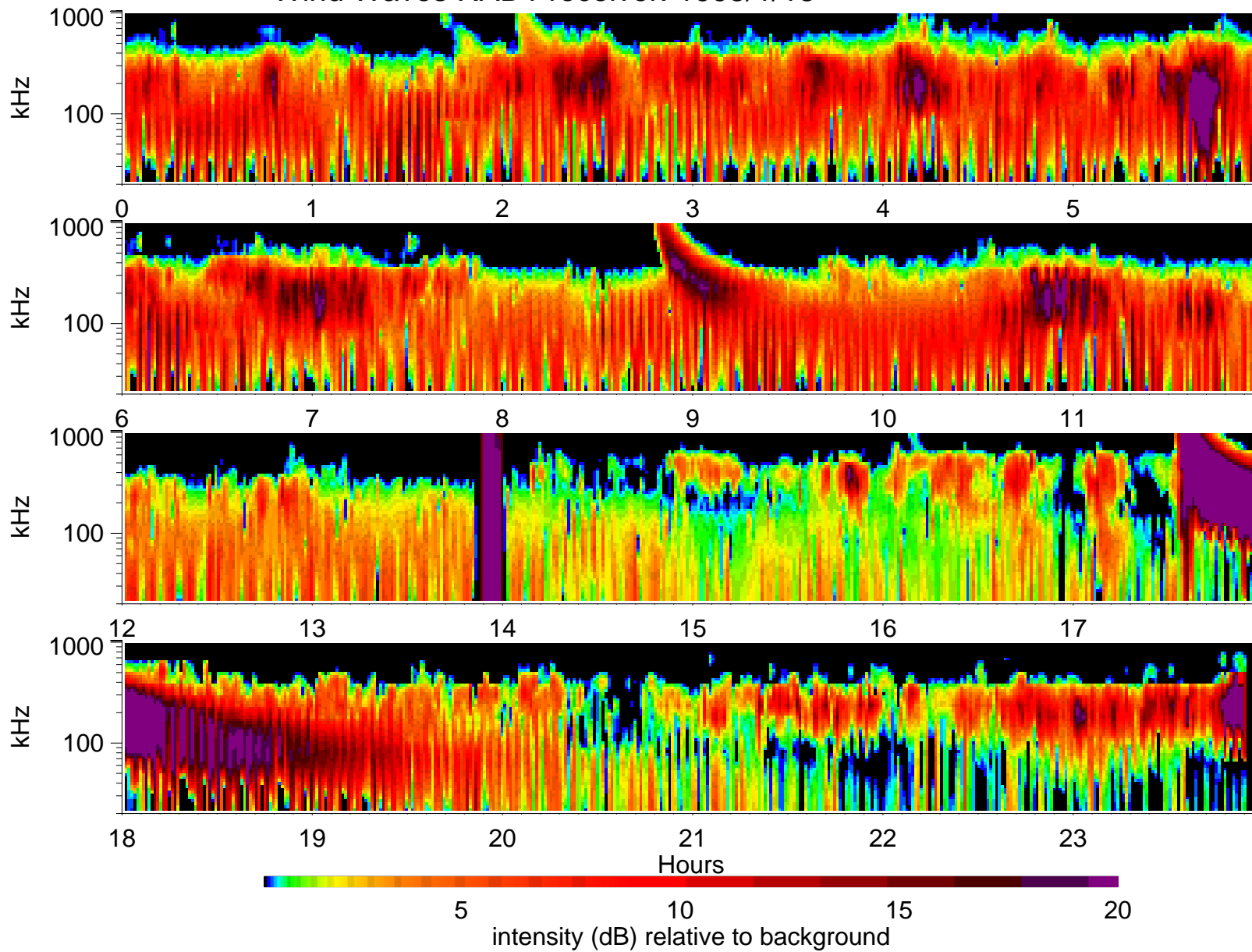
Wind Waves RAD1 receiver: 1995/1/18
