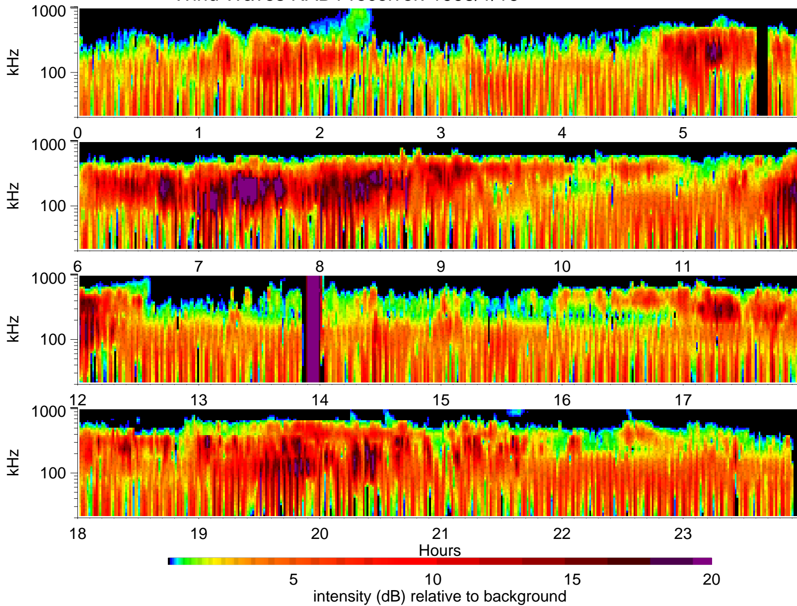
Wind Waves RAD1 receiver: 1995/1/16
