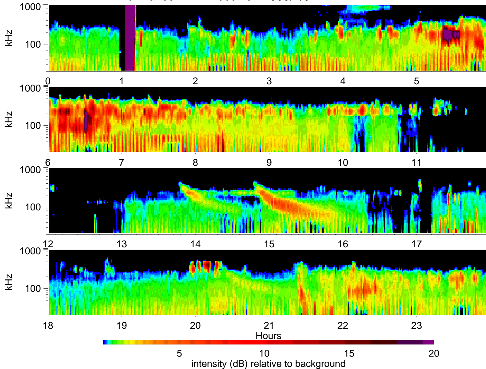
Wind Waves RAD1 receiver: 1995/1/9
