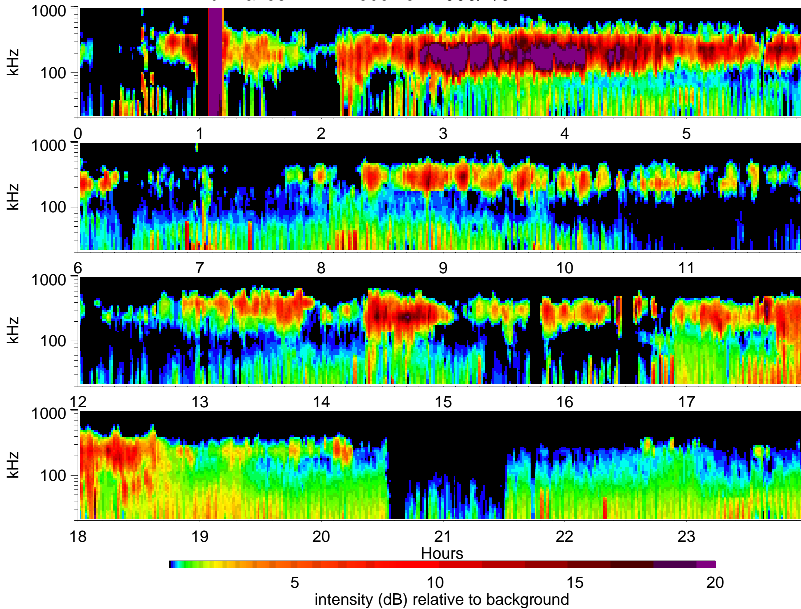
Wind Waves RAD1 receiver: 1995/1/8
