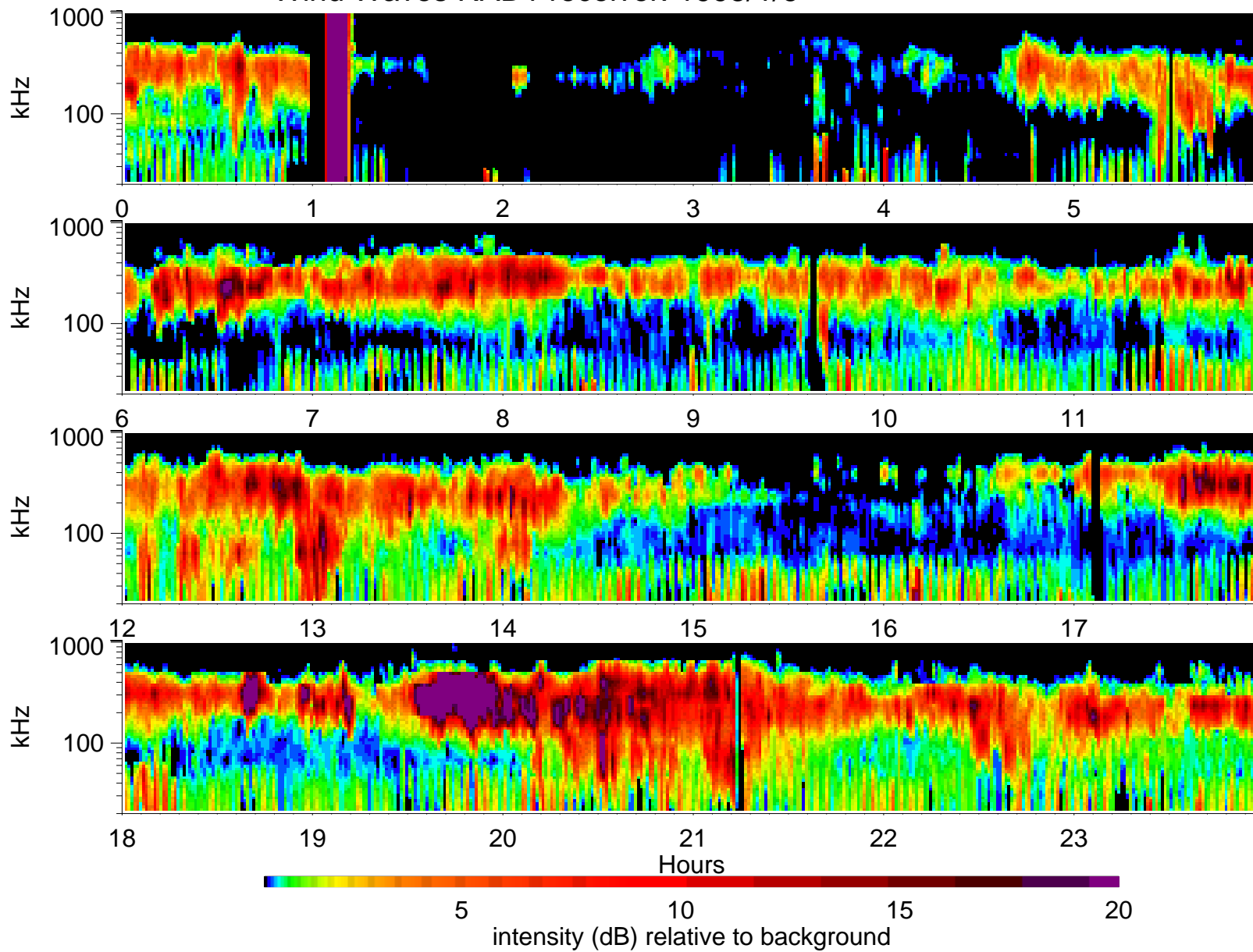
Wind Waves RAD1 receiver: 1995/1/6
