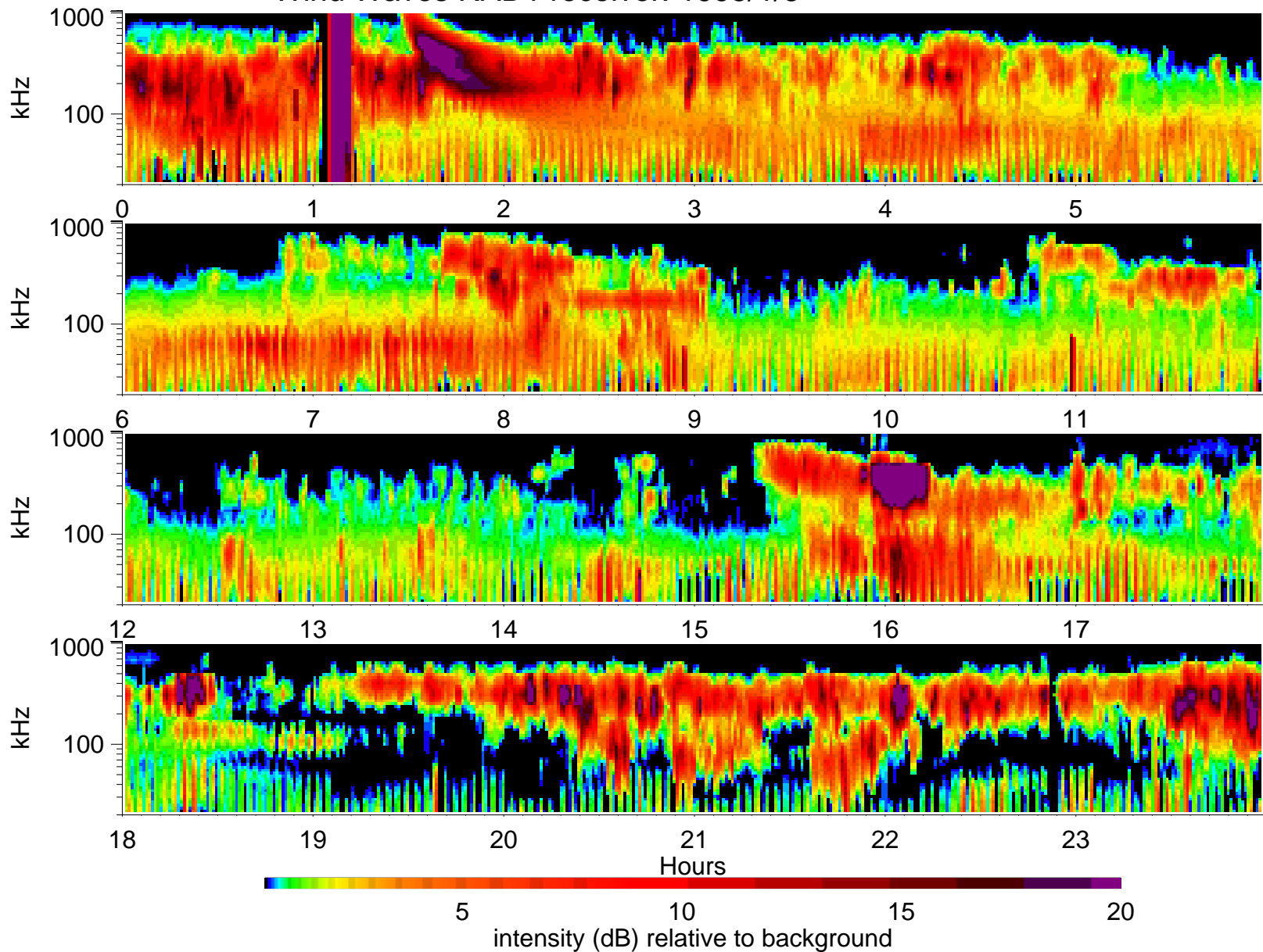
Wind Waves RAD1 receiver: 1995/1/3
