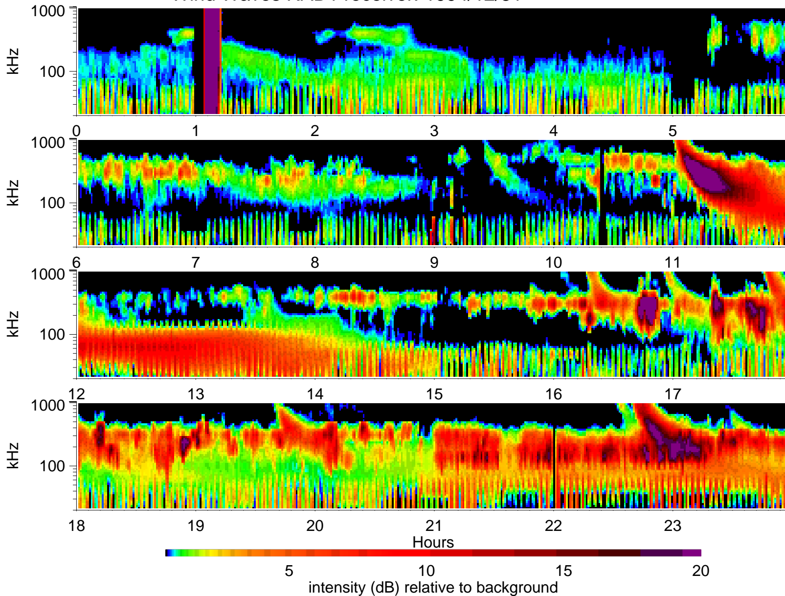
Wind Waves RAD1 receiver: 1994/12/31
