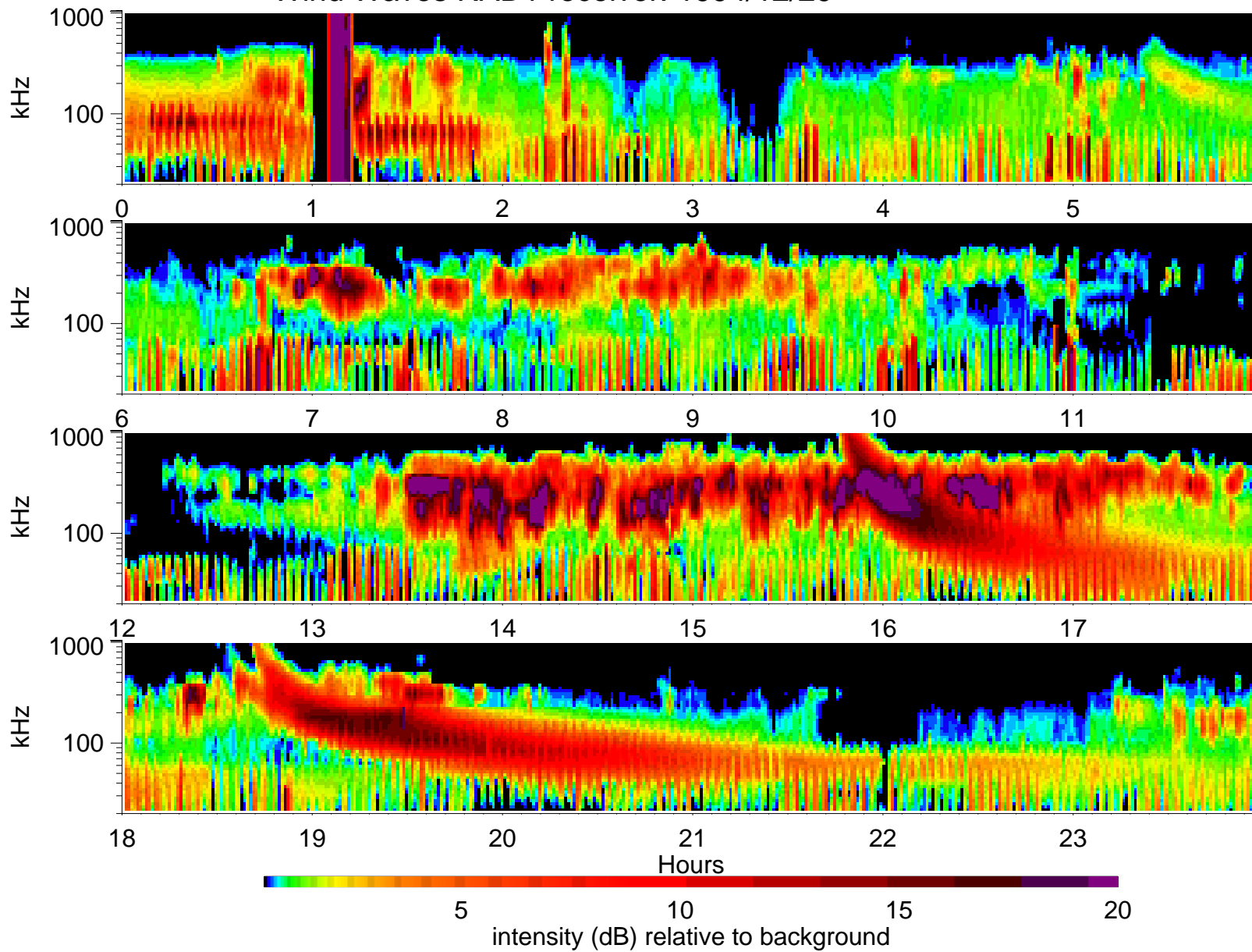
Wind Waves RAD1 receiver: 1994/12/29
