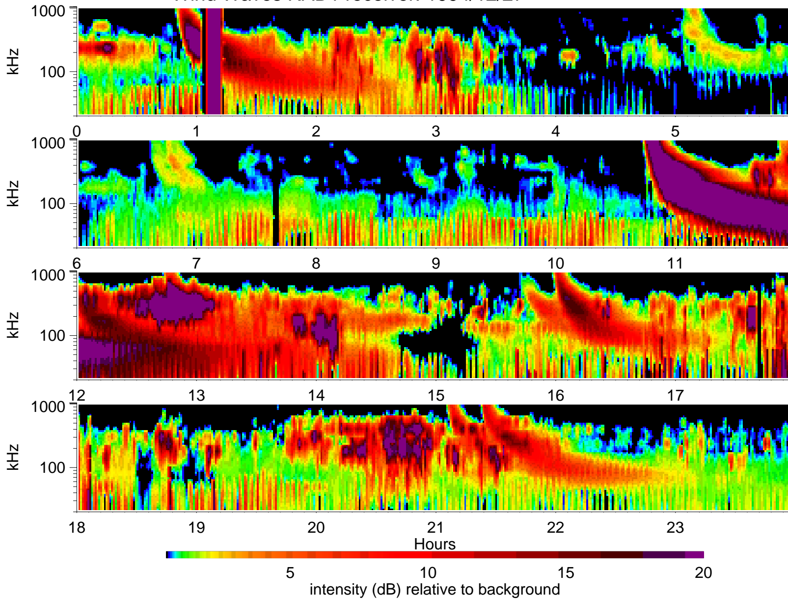
Wind Waves RAD1 receiver: 1994/12/27
