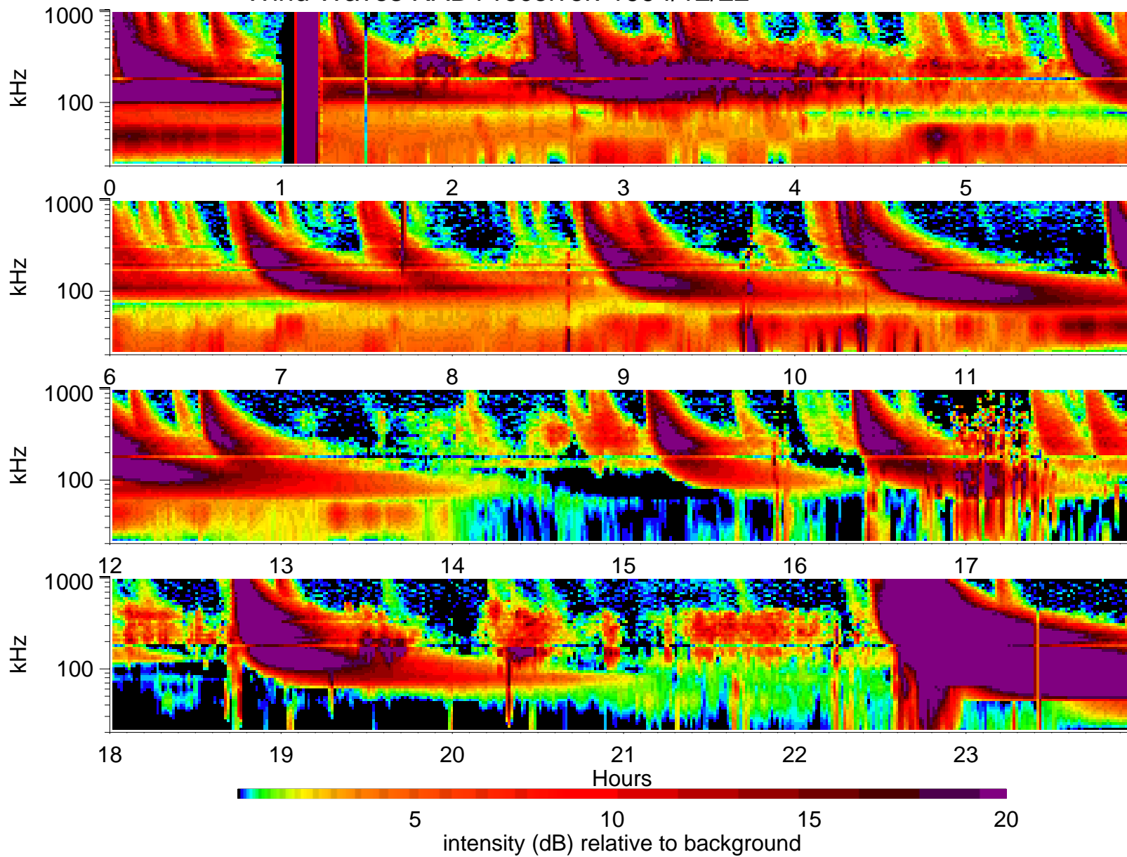
Wind Waves RAD1 receiver: 1994/12/22
