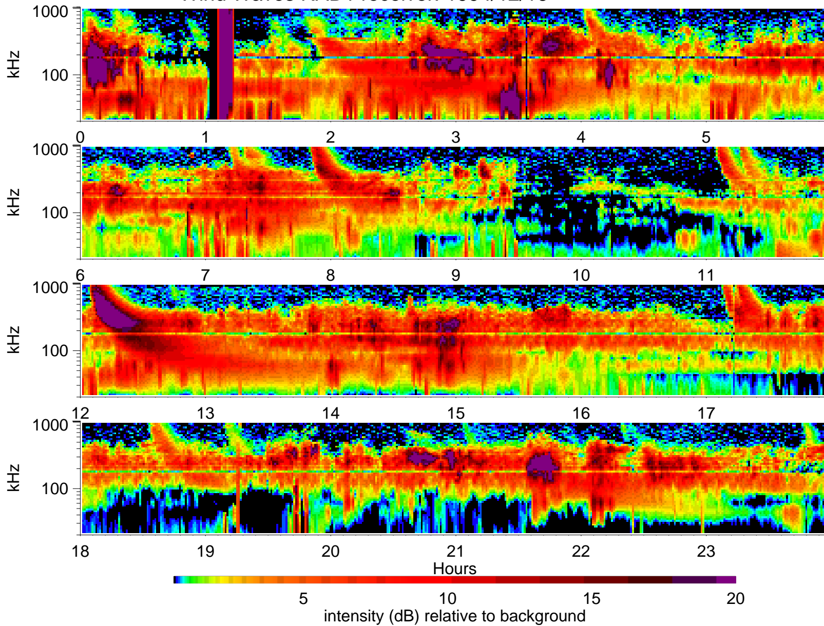
Wind Waves RAD1 receiver: 1994/12/16
