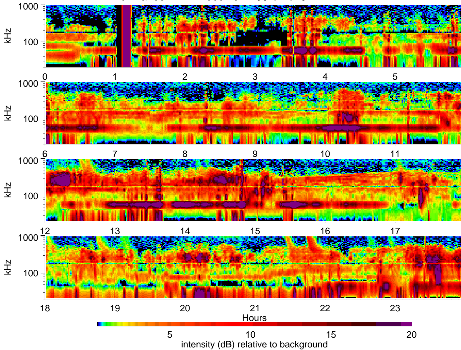
Wind Waves RAD1 receiver: 1994/12/15
