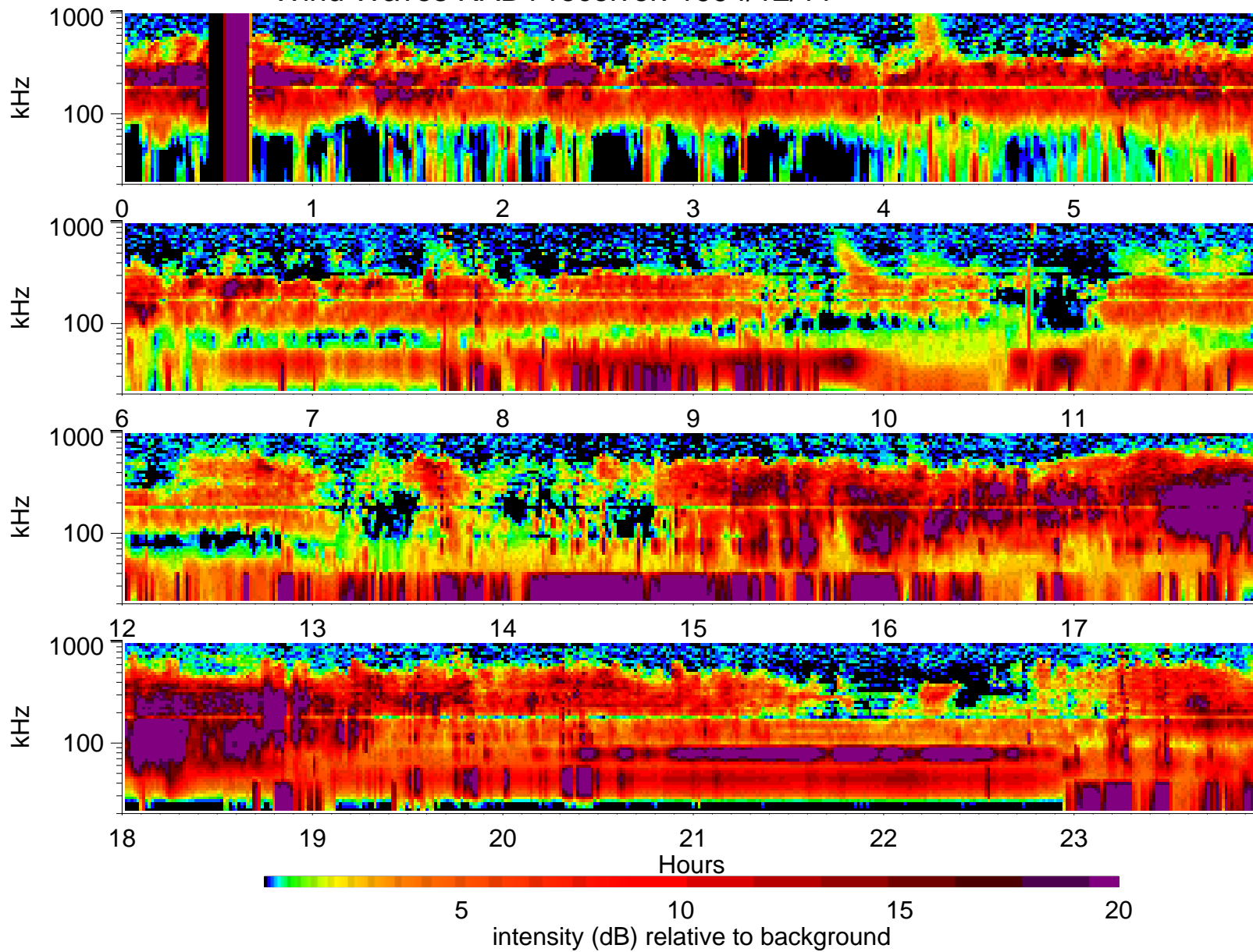
Wind Waves RAD1 receiver: 1994/12/11
