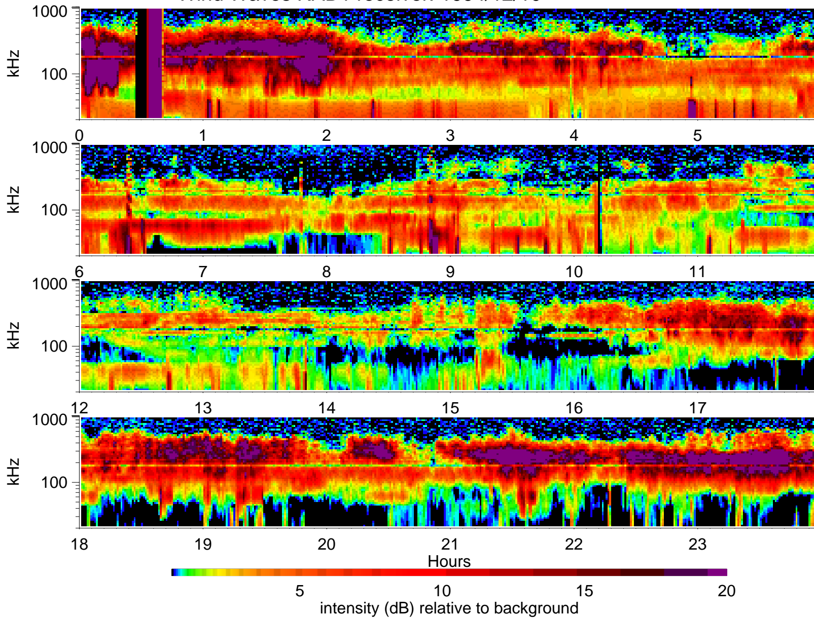
Wind Waves RAD1 receiver: 1994/12/10
